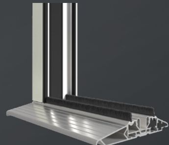
LOW THRESHOLD & FULL TRAY HEIGHT: 26.5mm
