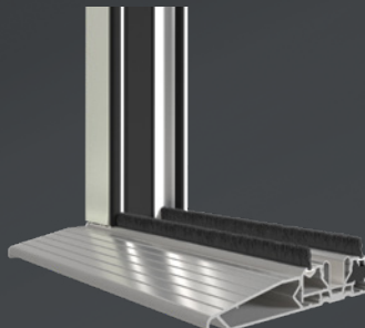
LOW THRESHOLD & HALF TRAY HEIGHT: 26.5mm
