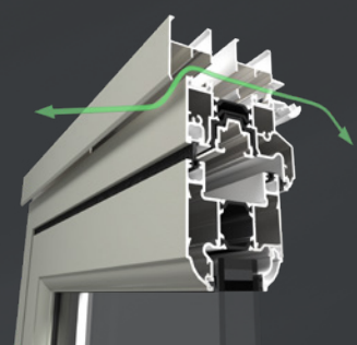
40MM ALUMINUM ADD-ON CONCEALED VENTILATION
